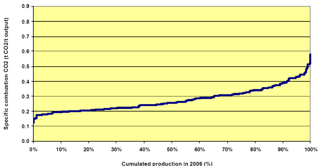
Figure 3 Specific combustion CO 2 emissions versus cumulated production for vertical kilns (CIBA, 2007)
