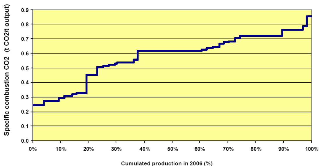
Figure 4 Specific combustion CO 2 emissions versus cumulated production for horizontal kilns (CIBA, 2007)
