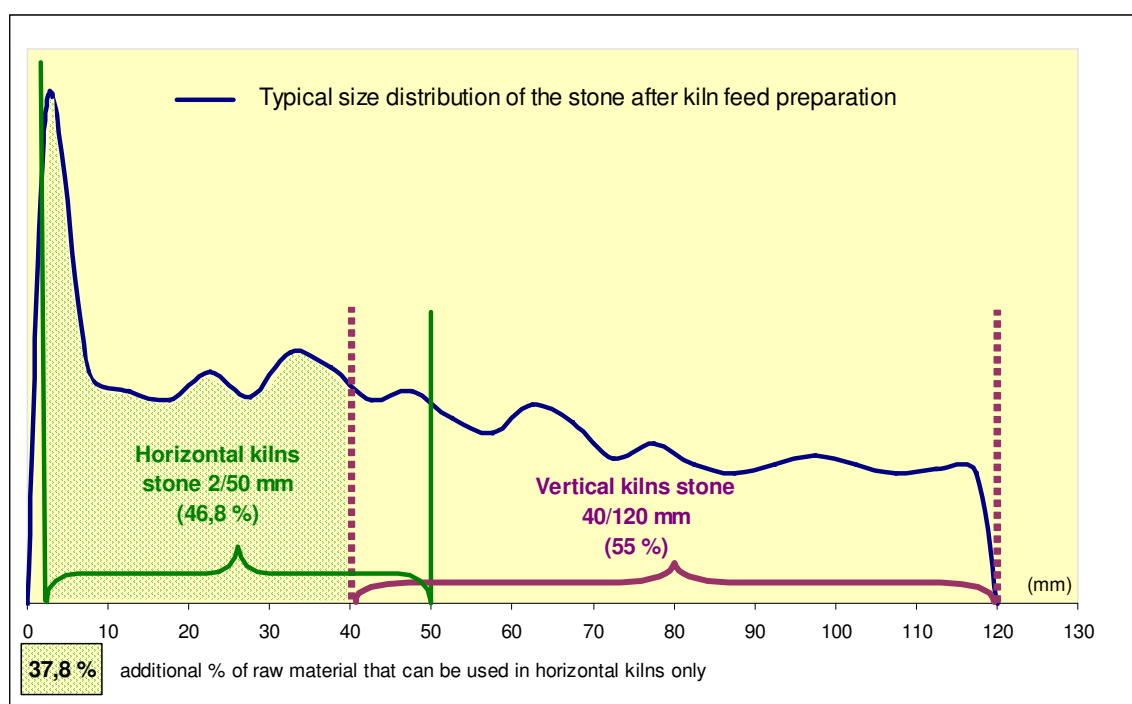
Figure 2 Typical size distribution of the stone after kiln feed preparation
